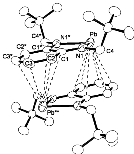
Figure 2. Molecular structure of dimeric 4 . Selected bond lengths [Å] and angles [°]: Pb–N1 2.180(4), N1–C1 1.373(7), N1–C4 1.457(6), C1–C1* 1.440(10); N1–Pb–N1* 75.4(2), Pb–N1–C1 115.3(3), Pb–N1–C4 121.8(4), C1–N1–C4 122.2(5).
